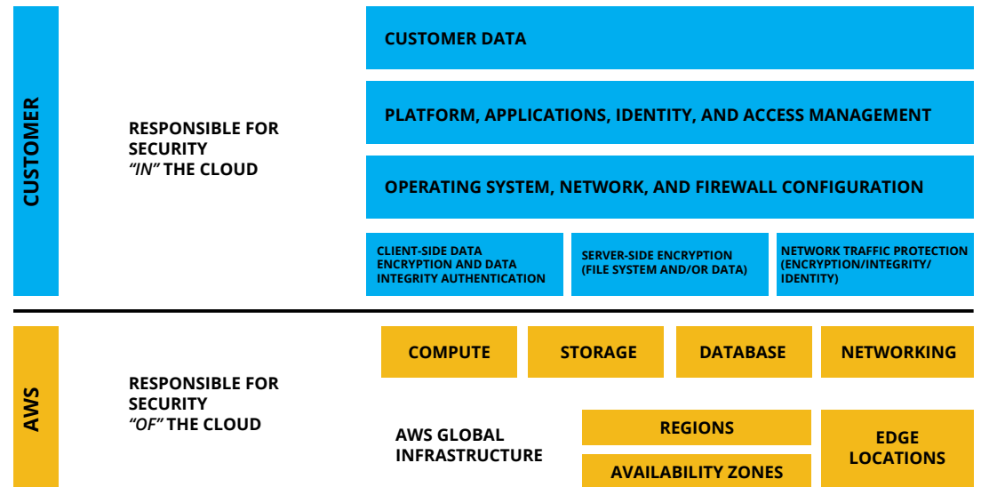
Figure 1. AWS Shared Responsibility Model ( https://aws.amazon.com/compliance/shared-responsibility-model )
