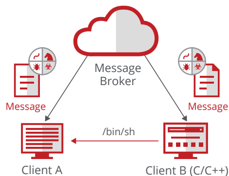
Figure 17. Command execution on a remote client via a message.
