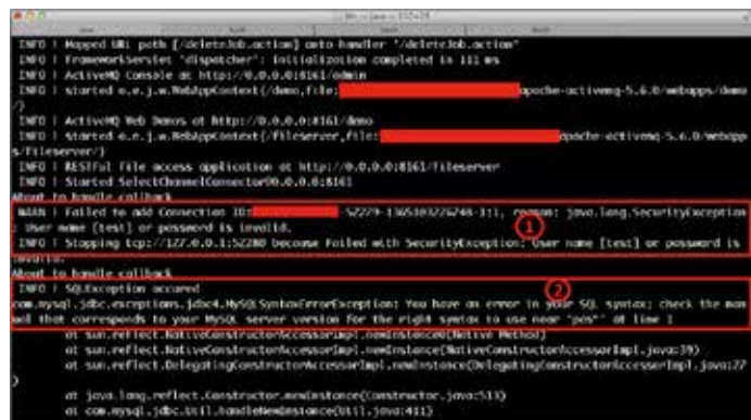
Figure 16. In the image, box 1 shows a regular authentication failure, box 2 shows SQL error indicating SQL injection vulnerability.
